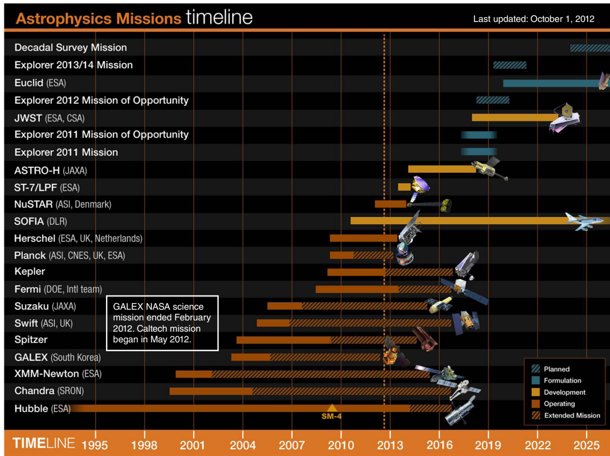
Figure 1. Astrophysics mission timeline through the early 2020s.
