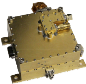
Figure 4 The RadioScience Beacon (RSB), flown on the GRAIL mission to the Moon, will allow calibration of the laser relative to the UltraStable Oscillator that drives the current MWI mission.
