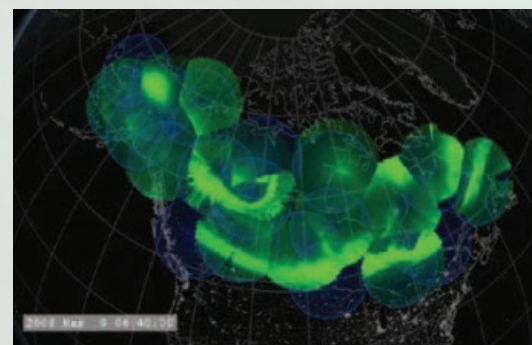
A collection of ground-based All-Sky Imagers (ASI) are an important component of NASA's Timed History of Events and Macroscale Interactions during Substorms (THEMIS) mission in understanding the interaction of the magnetosphere and aurora. This image highlights Canada and Alaska, in contrast to the main image highlighting the Southern Hemisphere. Credit: NASA/Goddard Space Flight Center Scientific Visualization Studio
