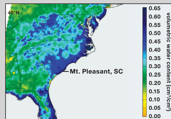
This image shows soil moisture conditions in the southeastern United States on October 5, 2015, as observed by SMAP's radiometer instrument. Most of South Carolina appears dark blue, due to widespread flooding caused by heavy tropical rainfall across the region. A record five-day (October 1-5) rainfall total of 27 inches (69 centimeters) was recorded in Mount Pleasant, SC.
