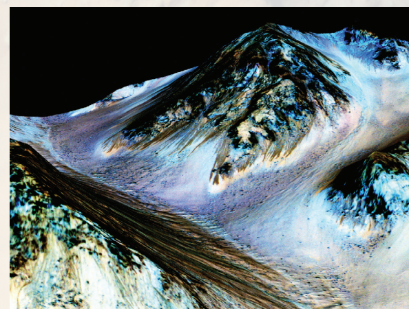
This false-color image, generated using imaging and topographical information from the High Resolution Imaging Science Experiment (HiRISE) camera on NASA's Mars Reconnaissance Orbiter (MRO), shows a different view of RSL (dark streaks) on Hale Crater.
