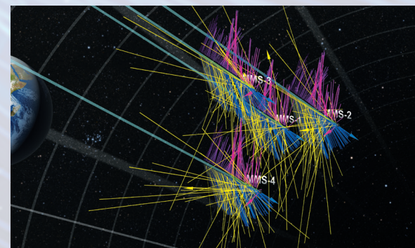
The image above was created using data collected by MMS near the height of the reconnection event. The arrows denote the direction of the magnetic field (magenta), electrons (yellow), and protons (blue) relative to the spacecraft position. The length of the blue and yellow vectors represent the particles' speed, while the length of the magenta vectors represent the strength of the magnetic fields. Note that the electrons (yellow arrows) are flying in all directions.
