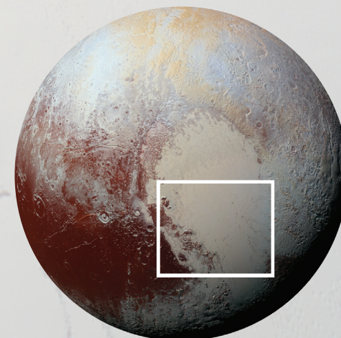
NASA's New Horizons spacecraft captured this enhanced color view of Pluto on July 14, 2015.
